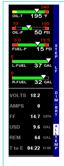
Vertical/Portrait mode
