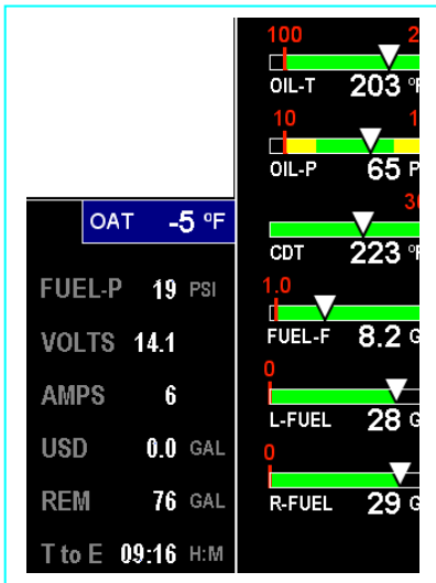
Horizontal/Landscape mode
